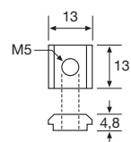
T-Slot Mounting Fixture Stainless Steel AISI 304 (2 units included)
